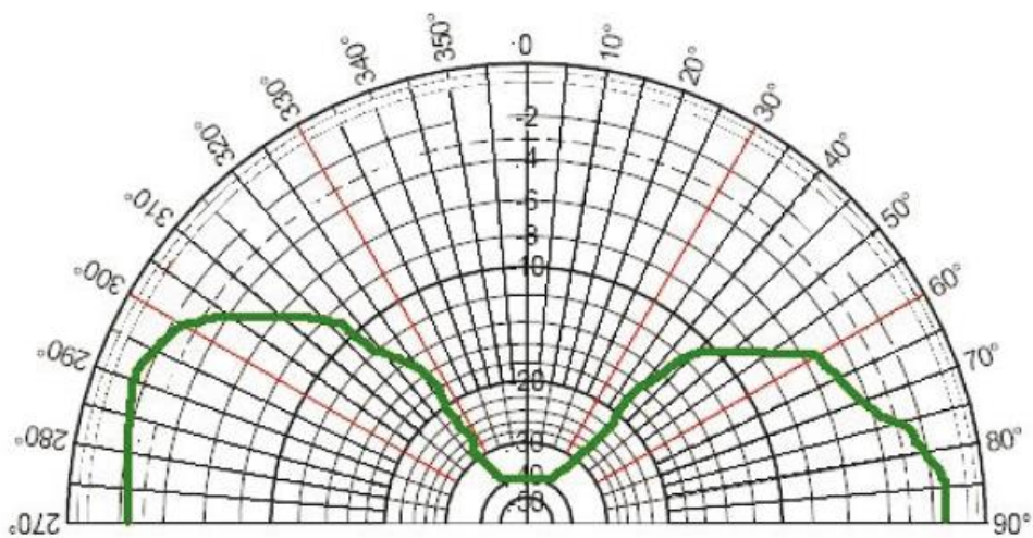
Elevation pattern (plano Z, Y or H-Plane)
