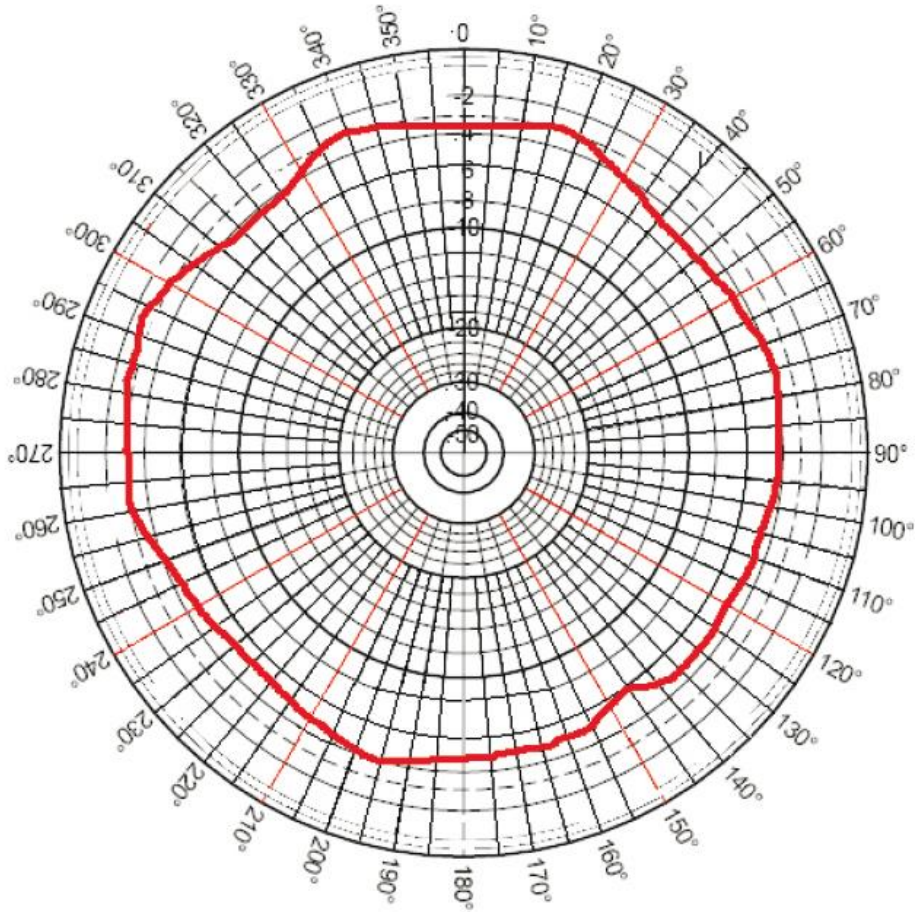
Diagrama acimutal (plano X, Y o E)
